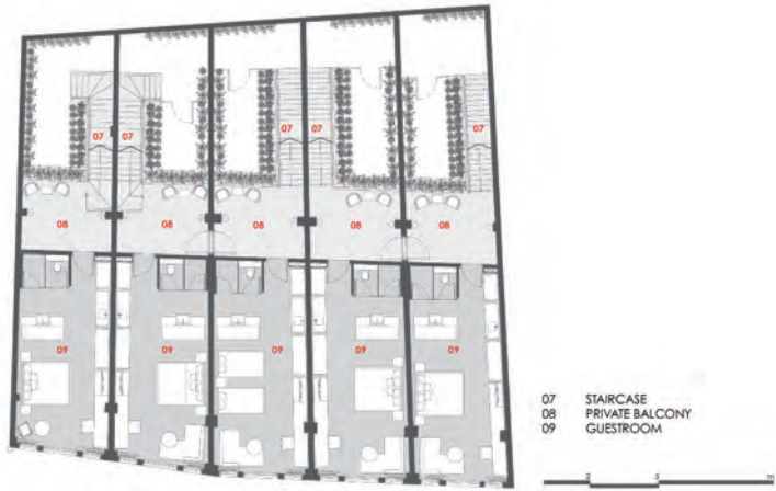
LTK FIRST FLOOR PLAN
